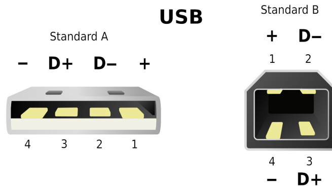
Figure 1 : Broches USB
